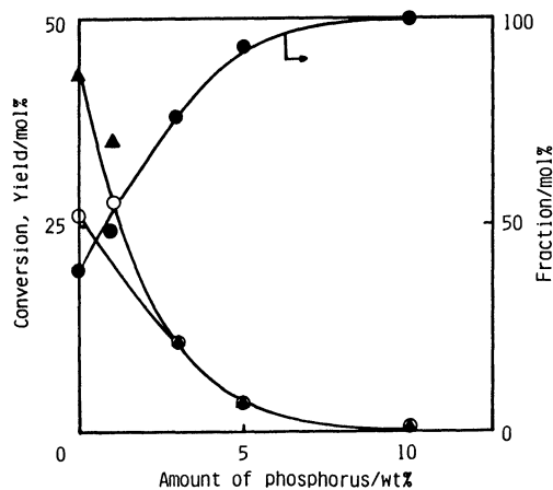
Fig. 5. Effect of amount of phosphorus added to HZSM-5 on conversion of ethylbenzene (▲), yield of diethylbenzene (○), and fraction of para-isomer in diethylbenzene produced (●) at 673 K and W/F=7.14 \text{ g h mol}^{-1} .
